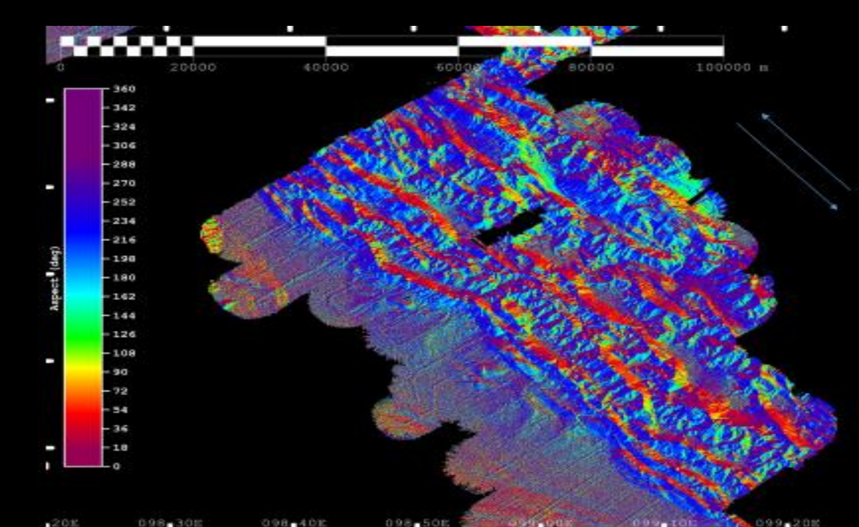
Figure 8b (below). 2D view of study site 2 using the slope aspect layer. Submarine ridges are represented in red, indicating they all have similar aspect (orientation).
