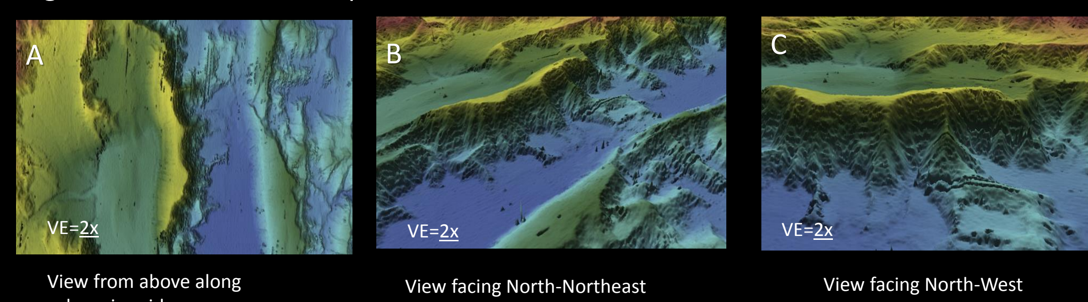
Figure 5. 3D views of scarp E
